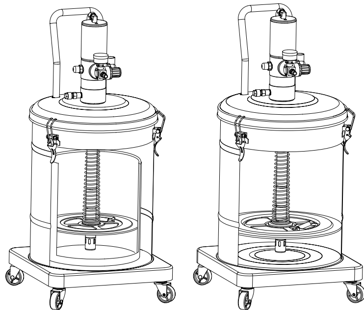
Standard barrel of grease can directly be put into the barrel
